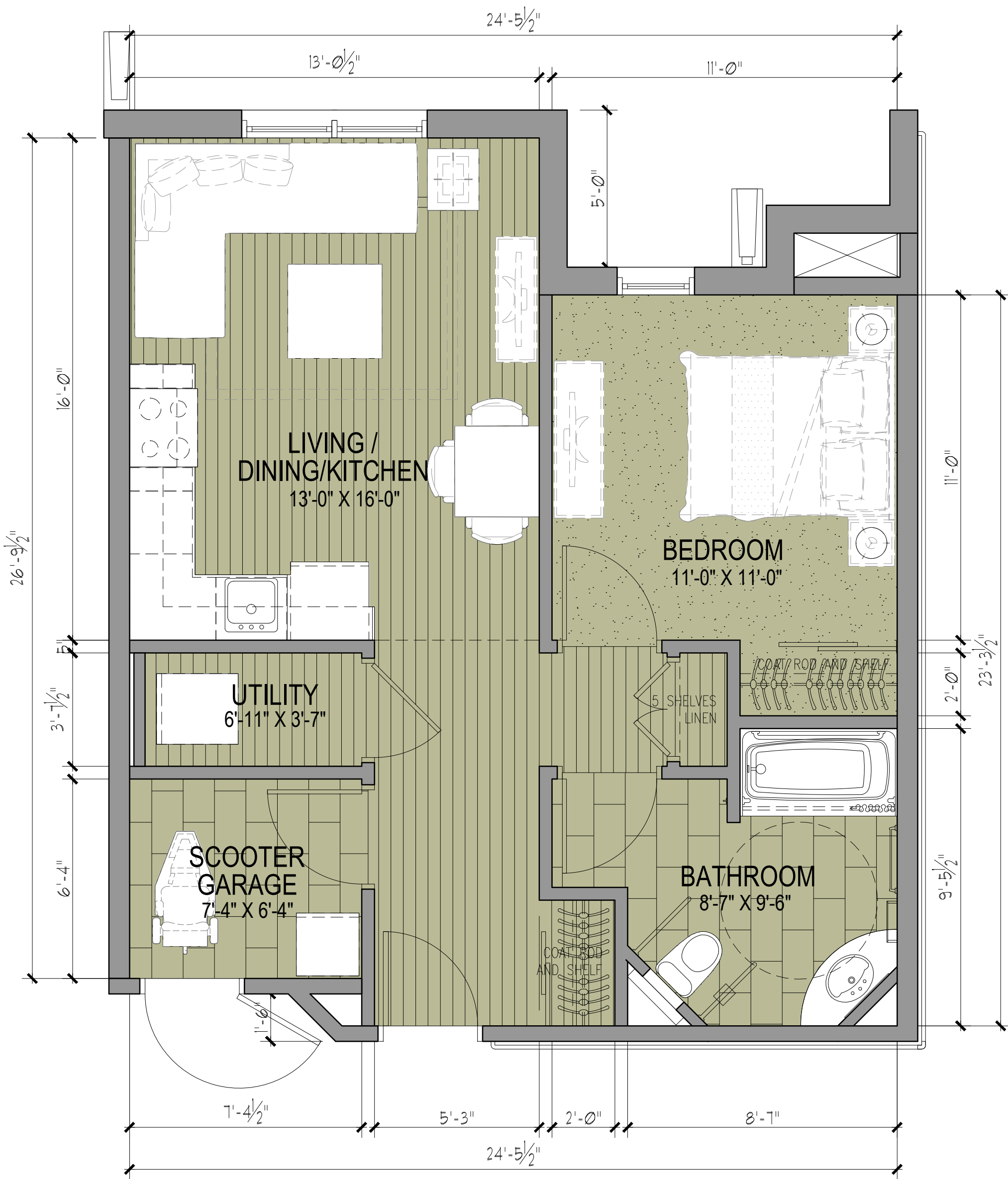
- TYP. SUITE - INDEPENDENT LIVING - 1-BEDRM. SUITE (8 UNITS) 650 sq.ft.
