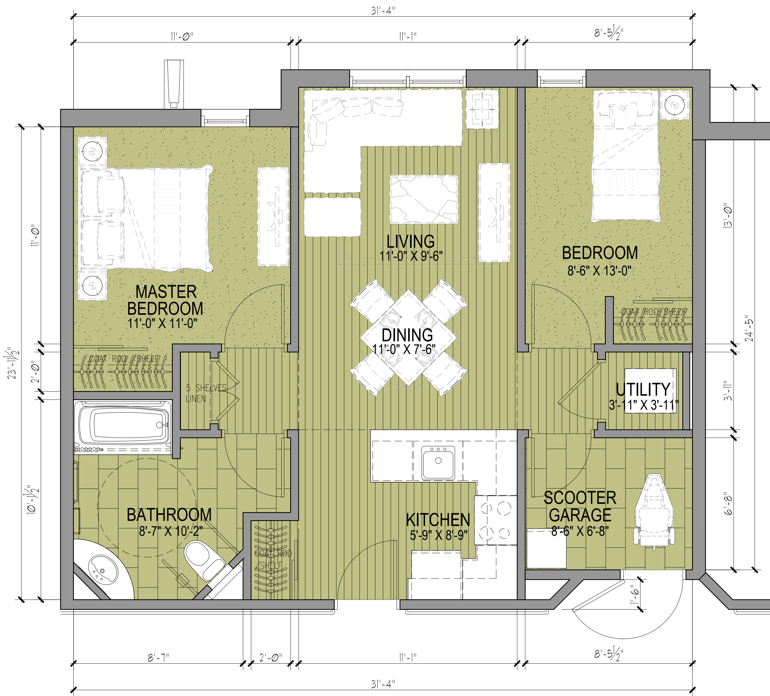
- TYP. SUITE - INDEPENDENT LIVING - 2-BEDRM. SUITE (4 UNITS) 803 sq.ft.
